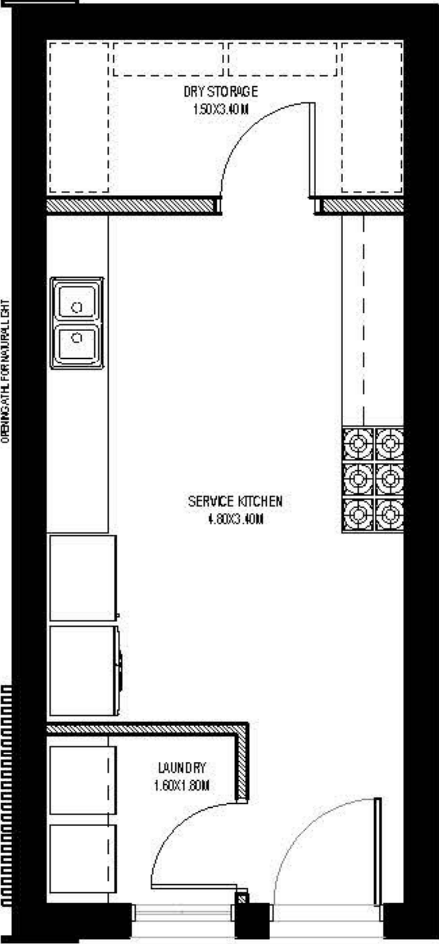
KITCHEN POD
