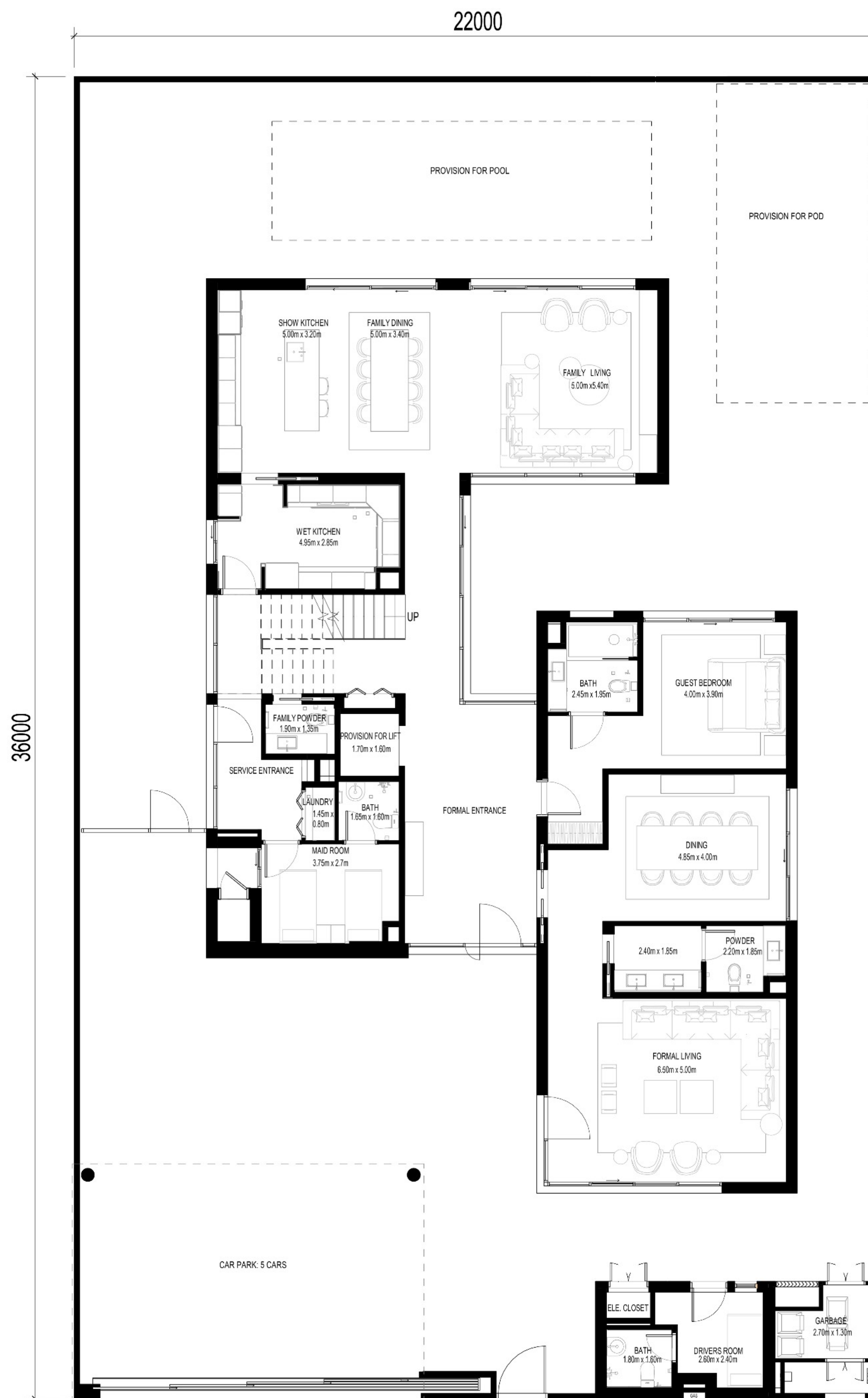
GROUND FLOOR
