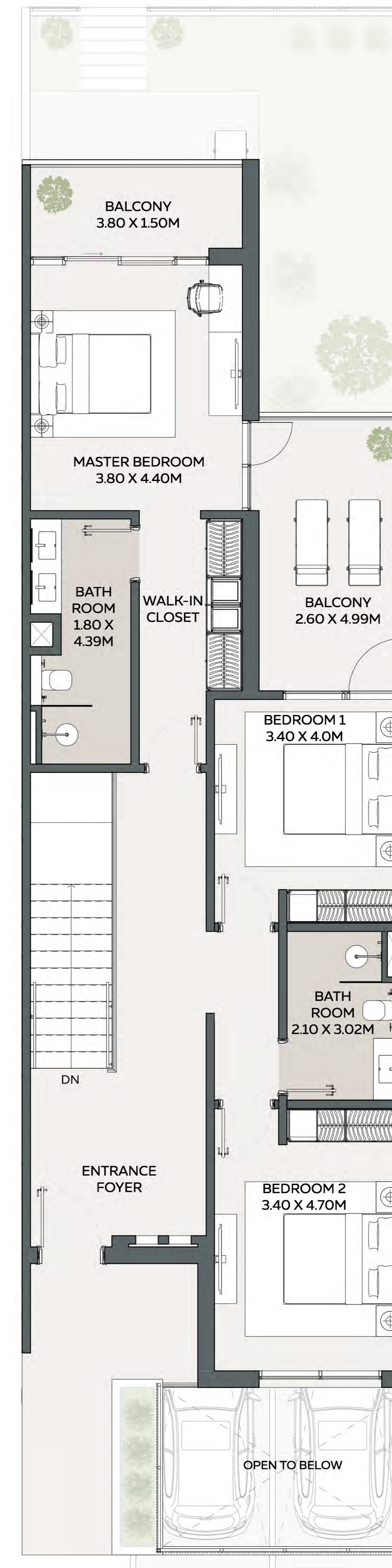
GROUND FLOOR
