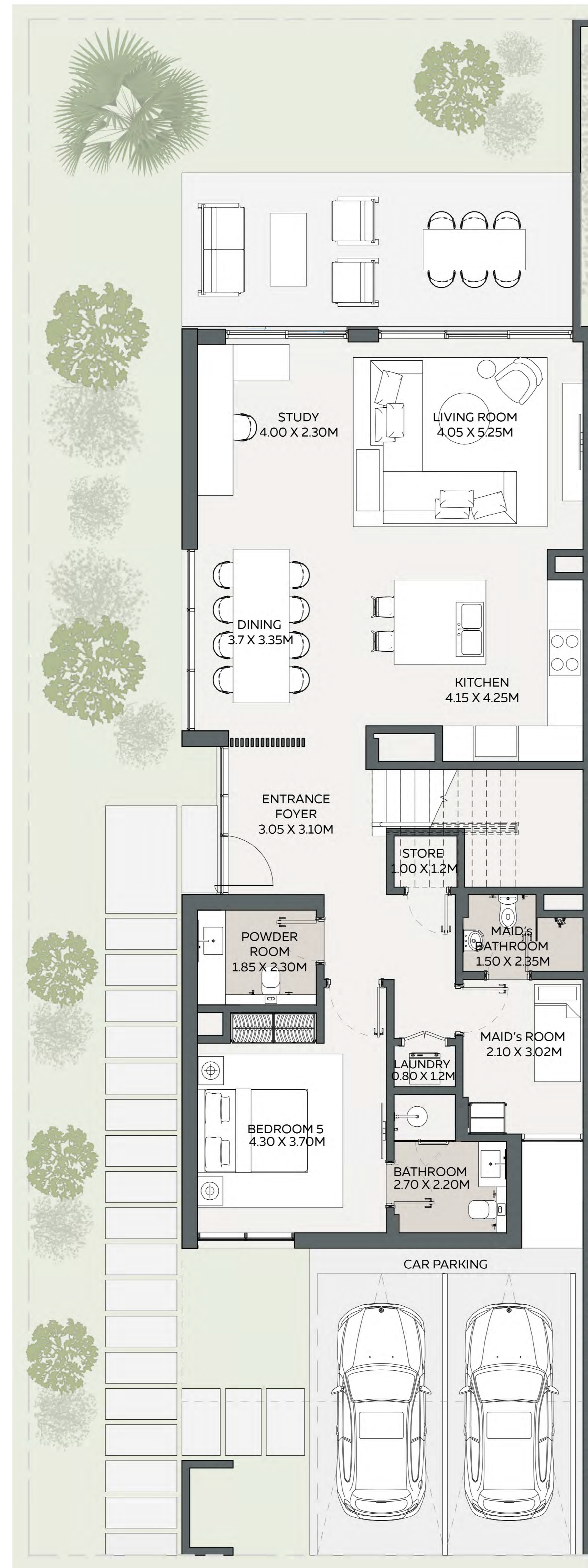
GROUND FLOOR
