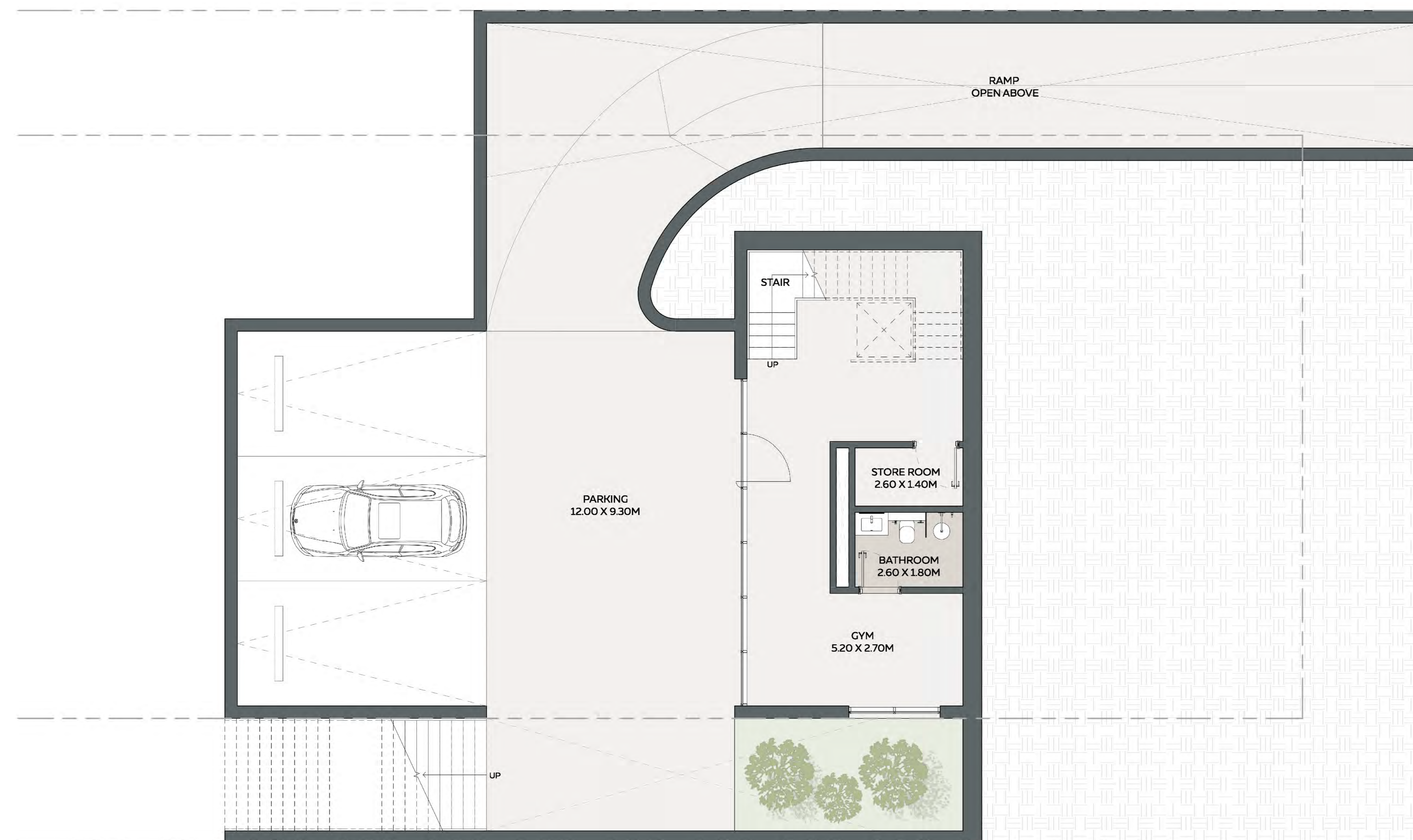
ROOF FLOOR
