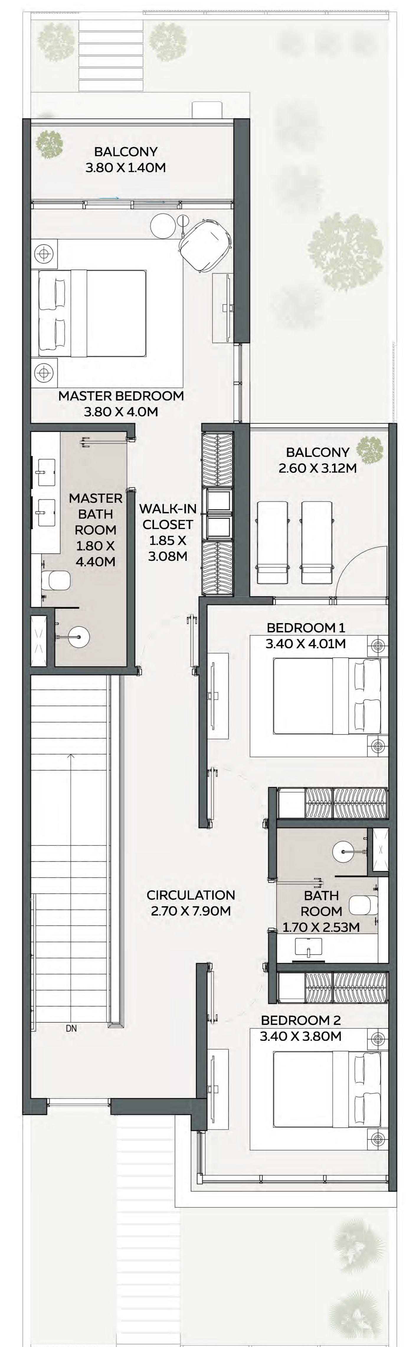
FIRST FLOOR
