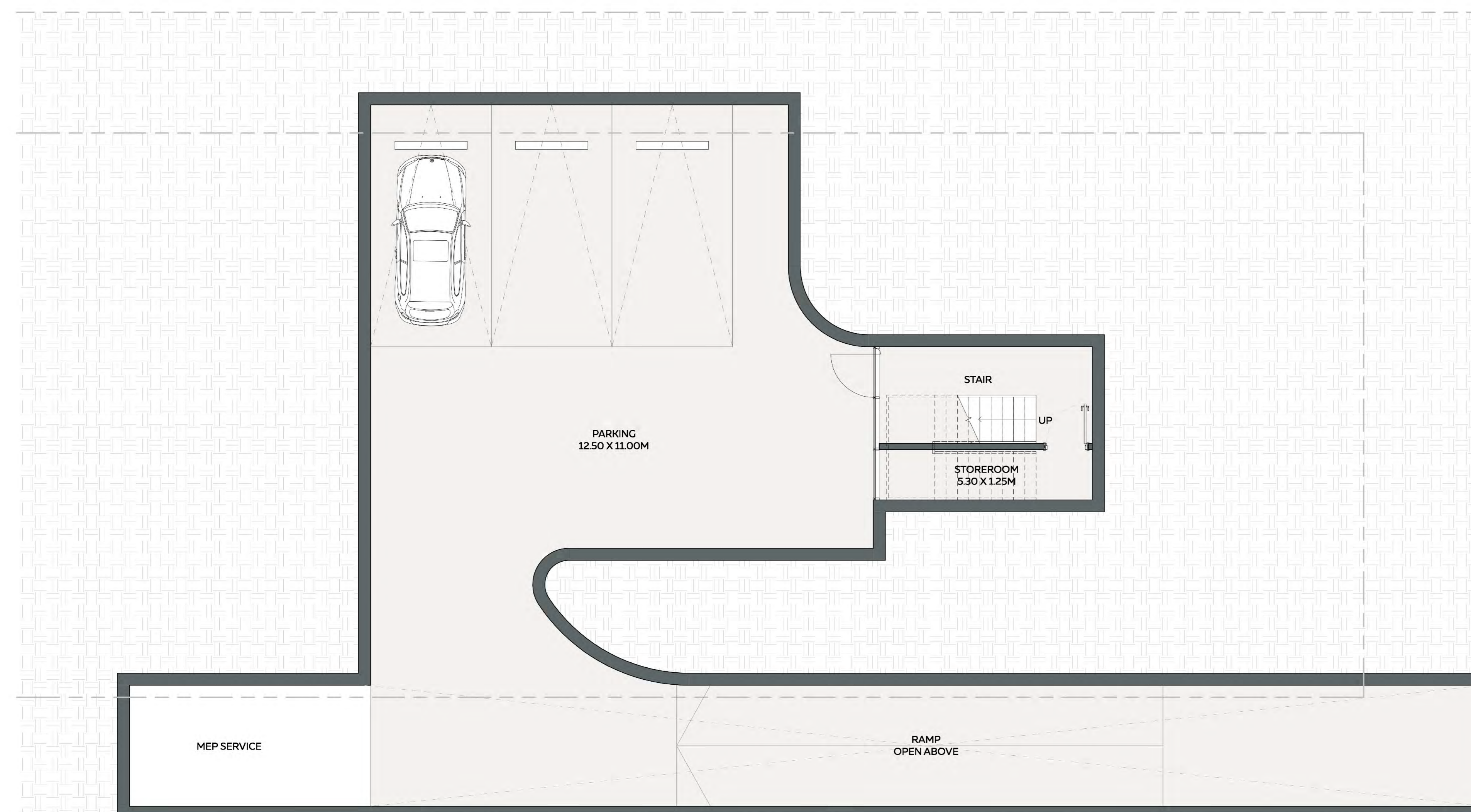
ROOF FLOOR
