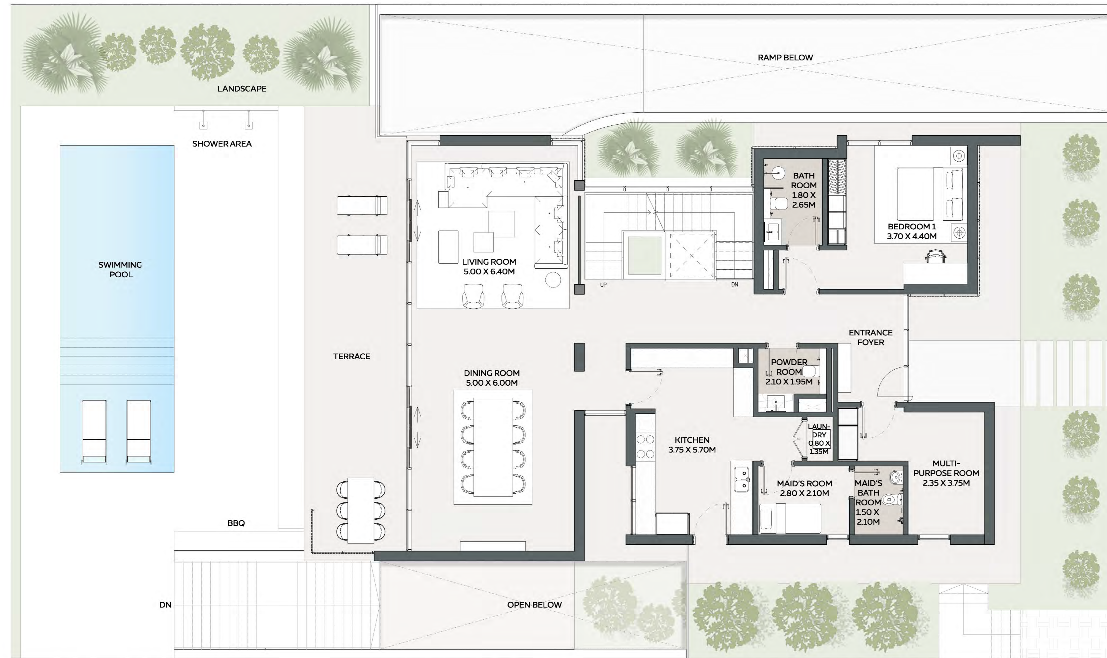
GROUND FLOOR
