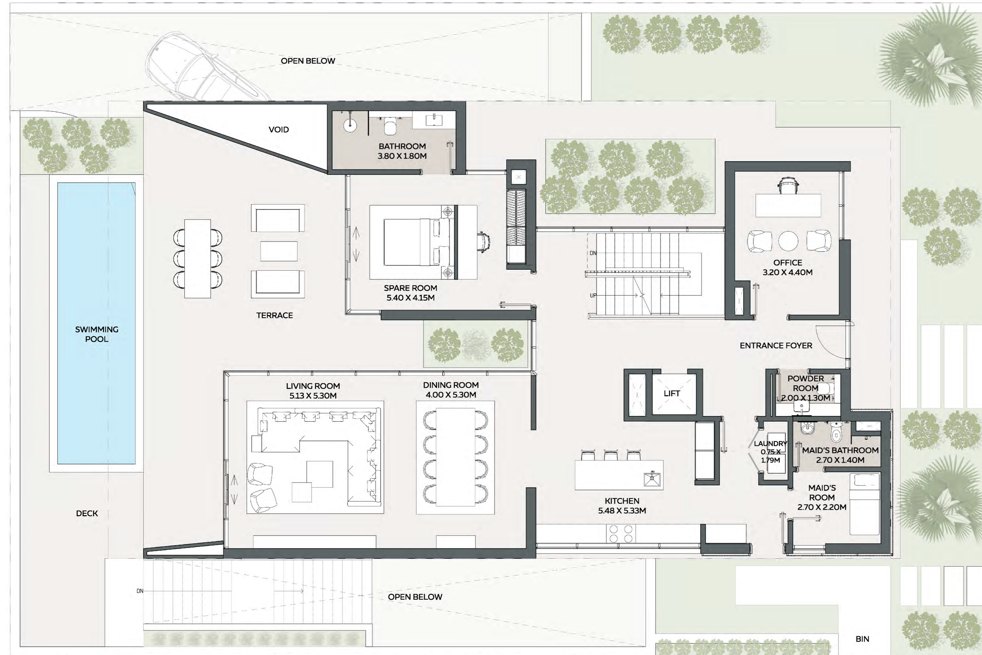
GROUND FLOOR
